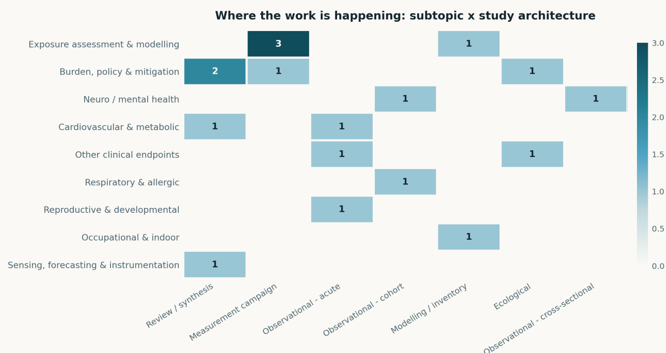
Fig. Subtopic × study-architecture cross-tabulation. The structural feature to note is the one this series has flagged repeatedly, and it is starkest today: the Exposure assessment and Sensing rows contain no health-endpoint linkage whatsoever, while every health-endpoint row is populated exclusively by designs that take exposure as a given input. Instrumentation and epidemiology remain methodologically siloed within this harvest.
