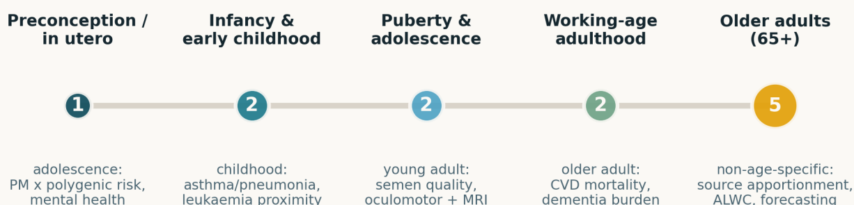
Fig. Life-course windows addressed. Counts are non-exclusive. The distribution is flat today: one adolescent, two childhood, two young-adult and two older-adult records, with the plurality (5) not age-specific because they are monitoring or source-apportionment work.
